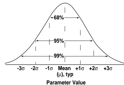
Figure 21. Normal Distribution.
